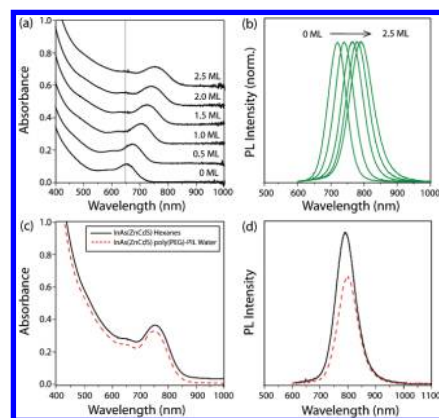
Figure 2. (a–b) Absorbance and PL of InAs(Zn 0.7 Cd 0.3 S) during shell growth from 0–2.5 monolayers (MLs). (c–d) Absorbance and PL ( \lambda_{\text{max}} = 795 \text{ nm} , fwhm = 82 nm) of InAs(Zn 0.7 Cd 0.3 S) in hexanes (black) and after ligand exchange with poly(PEG 12 )-PIL (red) in PBS at pH 7.4.
