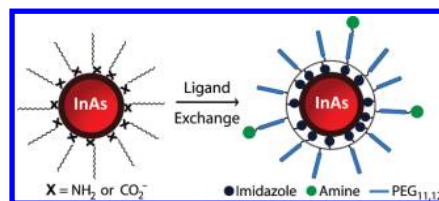
Figure 1. Ligand exchange of organic soluble QDs with poly(amino-PEG 11 ) 25 %-PIL to enable water solubilization.
